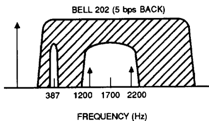
Figure 5. Half-Duplex Channel Assignments
