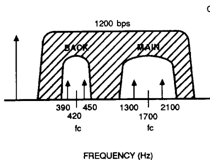
Figure 4. Full-Duplex Channel Assignments
