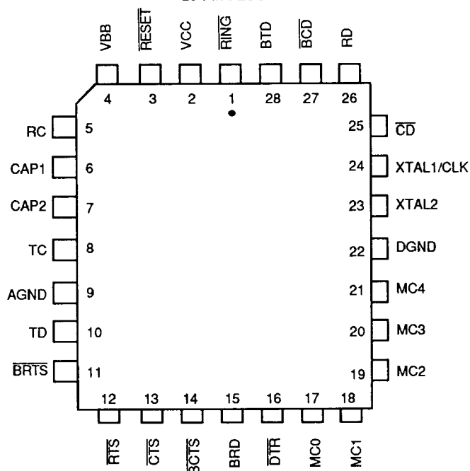
28-Pin PLCC
