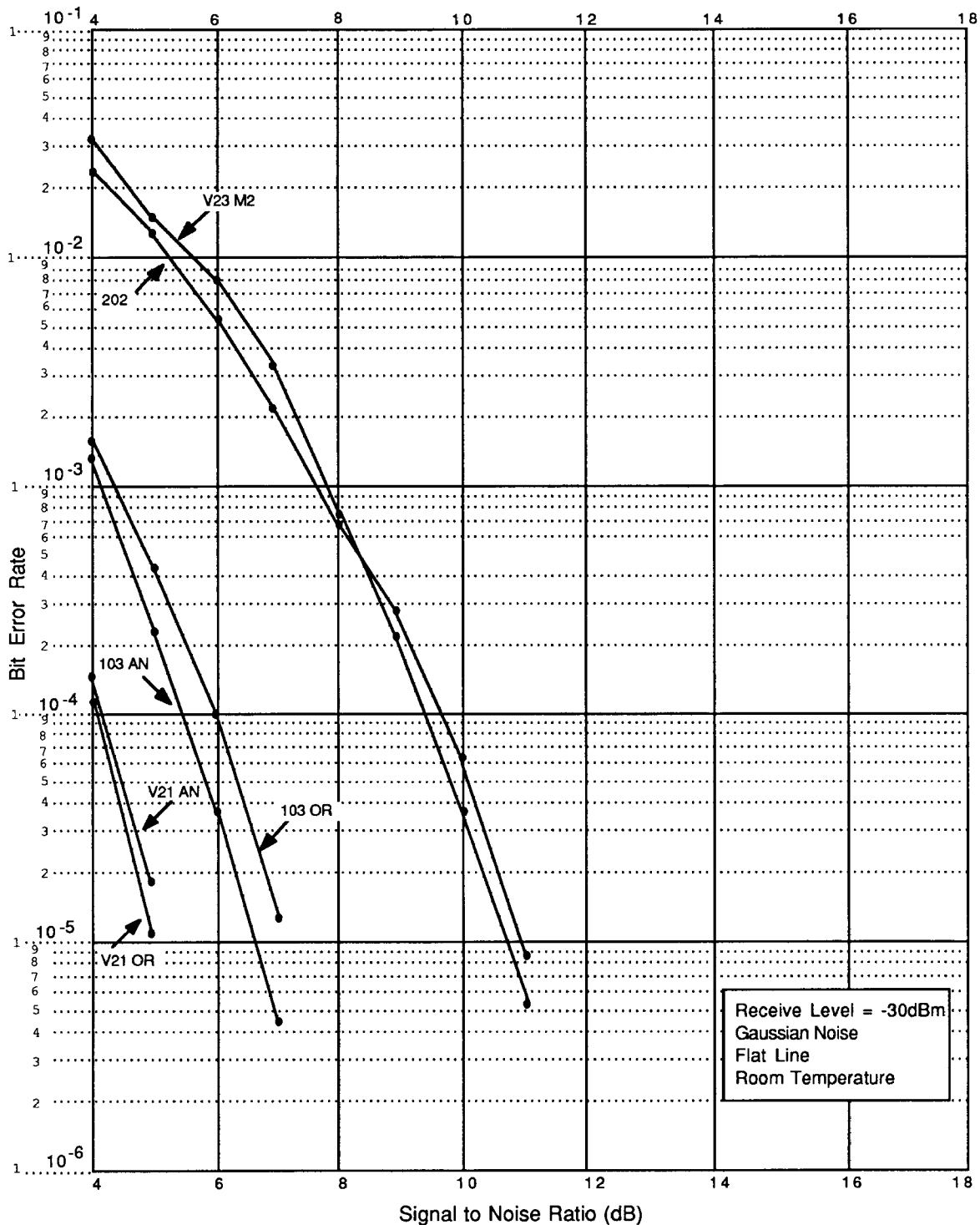
Figure 20. Am7910/11 Nominal Bit Error Rate
