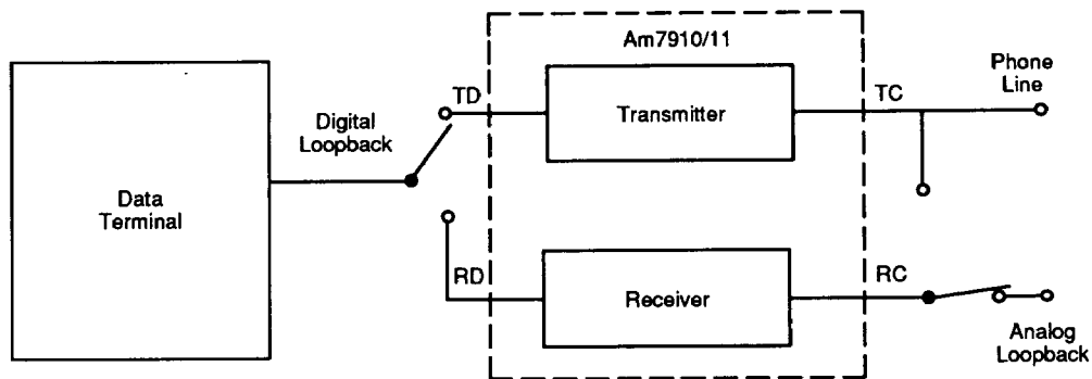
Figure 1. Analog Loopback
